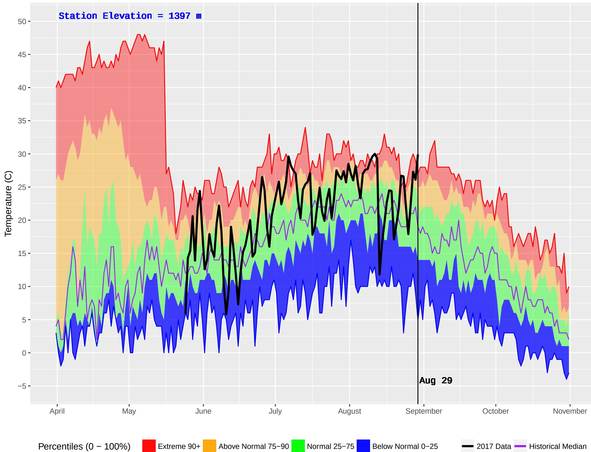
NANCY GREEN (407) : Historical (1992–2016) and Current (2017) Noon Temperature
